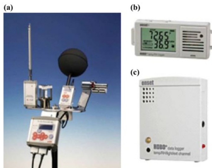
14 Figures: (a) LSI-Lastem thermal comfort logger (LSI TC); (b) Hobo temp/RH logger (HOBO-1), and (c) Hobotemp/RH/Light/External logger (HOBO-2)
